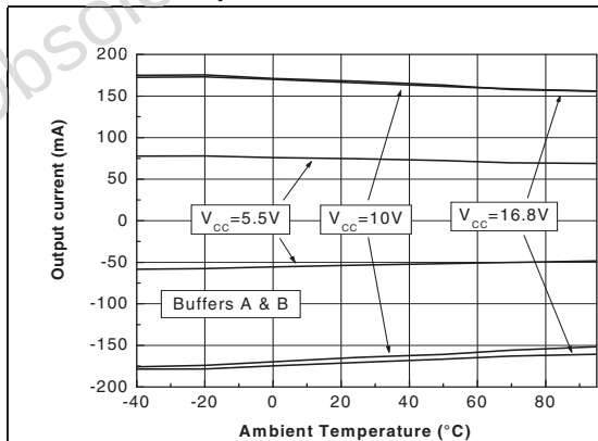
Figure 6. Output current capability vs. temperature
