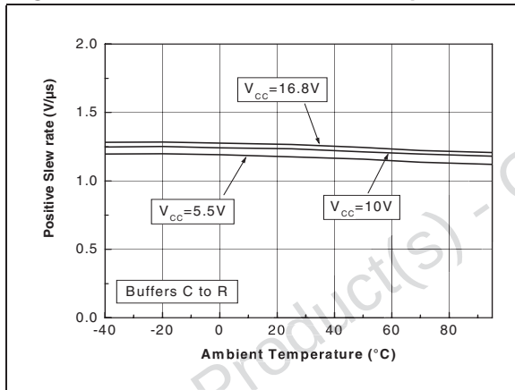
Figure 22. Positive slew rate vs. temperature
