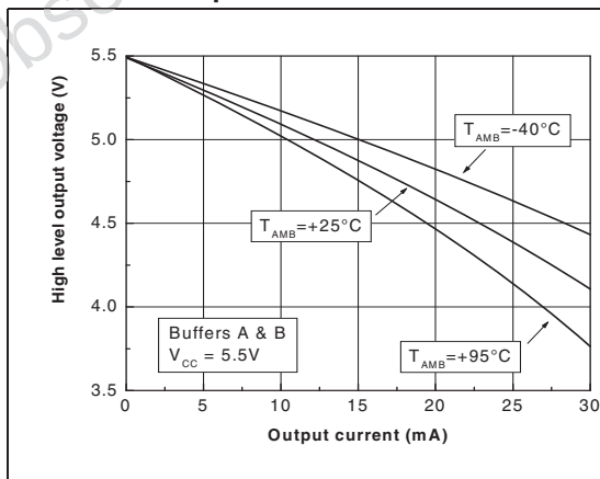
Figure 12. Voltage output high (VOH) vs. output current - buffers A & B
