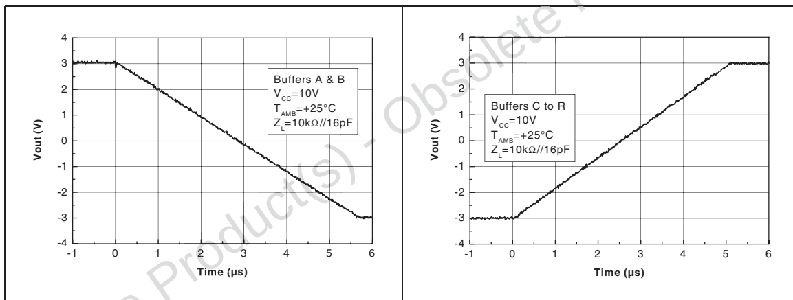
Figure 28. Large signal response - buffers A & B Figure 29. Large signal response - buffers C to R
