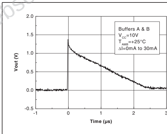
Figure 36. Output voltage response to current transient - buffers A & B
