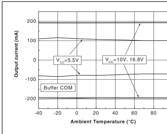
Figure 8. Output current capability vs. temperature
