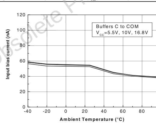
Figure 5. Input current ( I_{IB} ) vs. temperature
