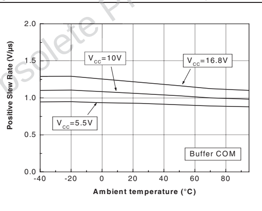
Figure 22. Positive slew rate vs. temperature
