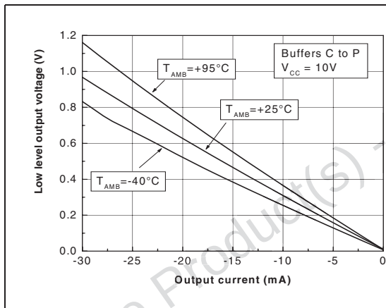
Figure 16. Voltage output low ( V_{OL} ) vs. output current - buffers C to P
