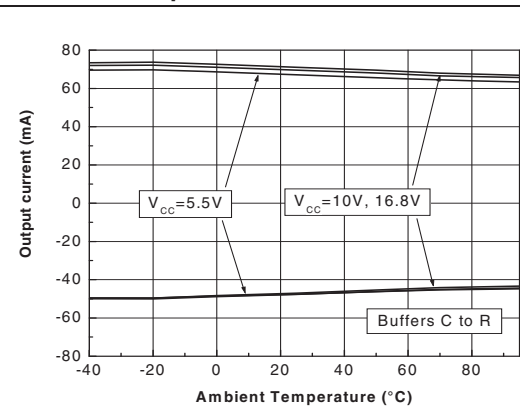
Figure 7. Output current capability vs. temperature
