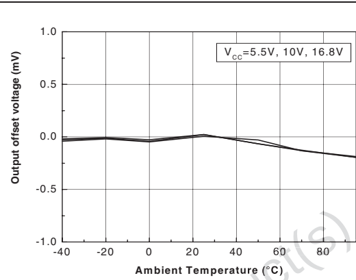
Figure 3. Output offset voltage (eq. V_{IO} ) vs. temperature
