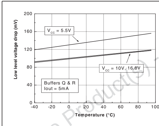
Figure 10. Low level voltage drop vs. temperature
