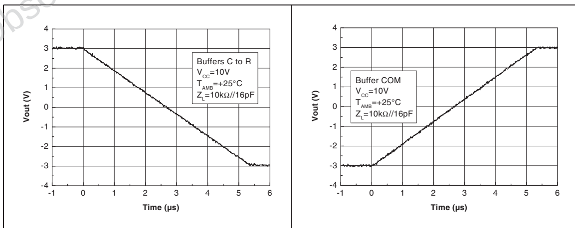
Figure 30. Large signal response - buffers C to R Figure 31. Large signal response - buffer COM
