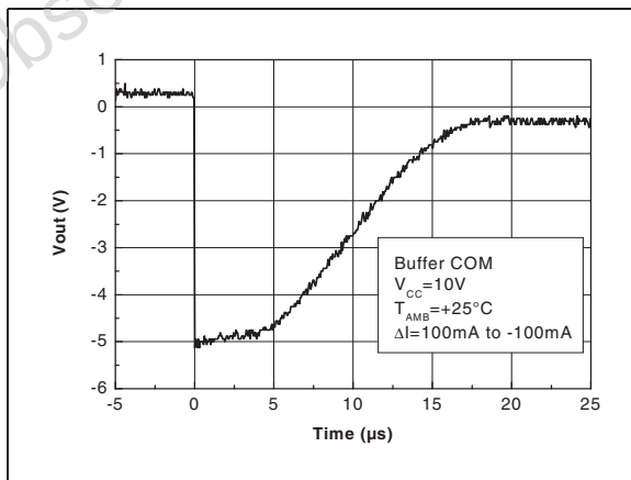
Figure 42. Output voltage response to current transient - buffer COM
