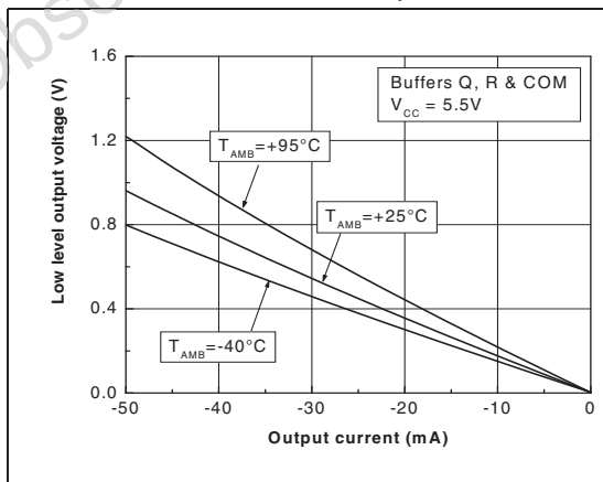
Figure 18. Voltage output low ( V_{OL} ) vs. output current - buffer Q, R & COM
