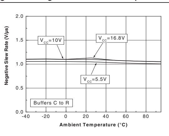
Figure 24. Negative slew rate vs. temperature
